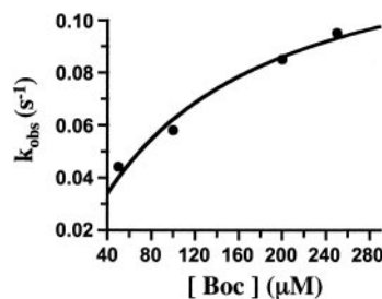
FIG. 2. The observed first-order rate constants for covalent modification of Tp47 as a function of the concentrations of BOCILLIN FL. The equation that defines this plot is described under "Experimental Procedures."
